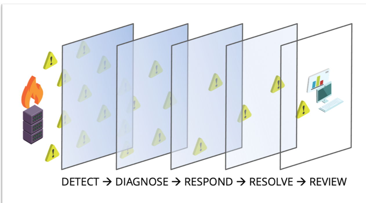
Figure 1: Five gates of AIOps solutions, designed to buffer alert noise and decrease time to resolution.
